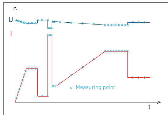
Waveform generated by the LIST function in CC mode with synchronized measurement of time, voltage, and current
