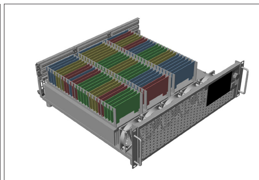
Example: 1 PMLA LP device with 3 cooling units, fully assembled with mixed load channels
